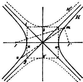
C. 1874. Hyperbola v geometrii.
